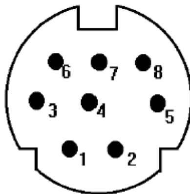
CONECTOR MINI-DIN 8 PINS
