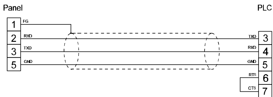
figure 1. Cable diagram
